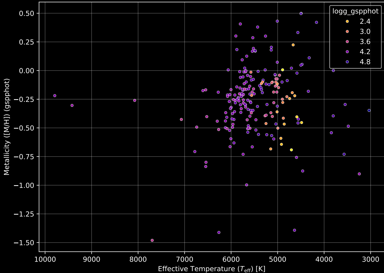
APOGEE DR17 Field: [162+60_MGA] Stellar Population Parameters (n= 205)
