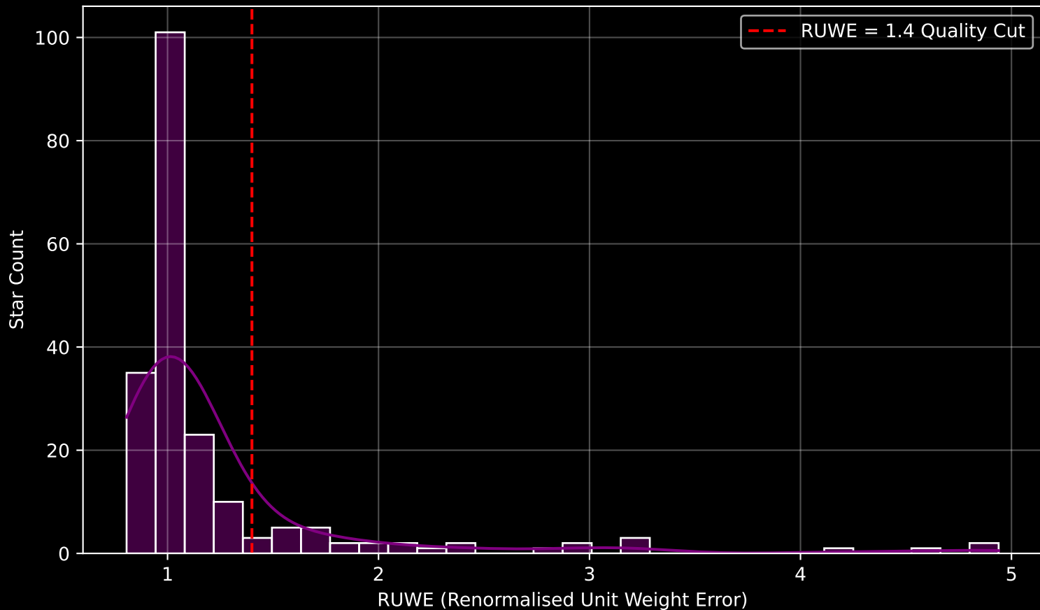
GAPOGEE DR17 Field [162+60_MGA] RUWE Distribution (n= 201)
