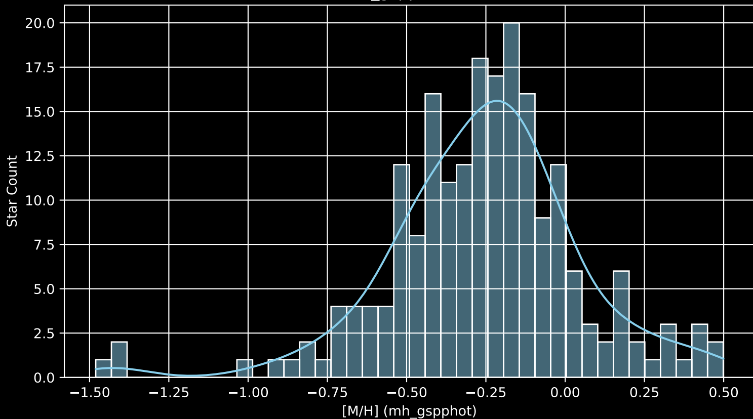
APOGEE DR17 Field: [162+60_MGA [M/H] (mh_gspphot) (n= 205)
