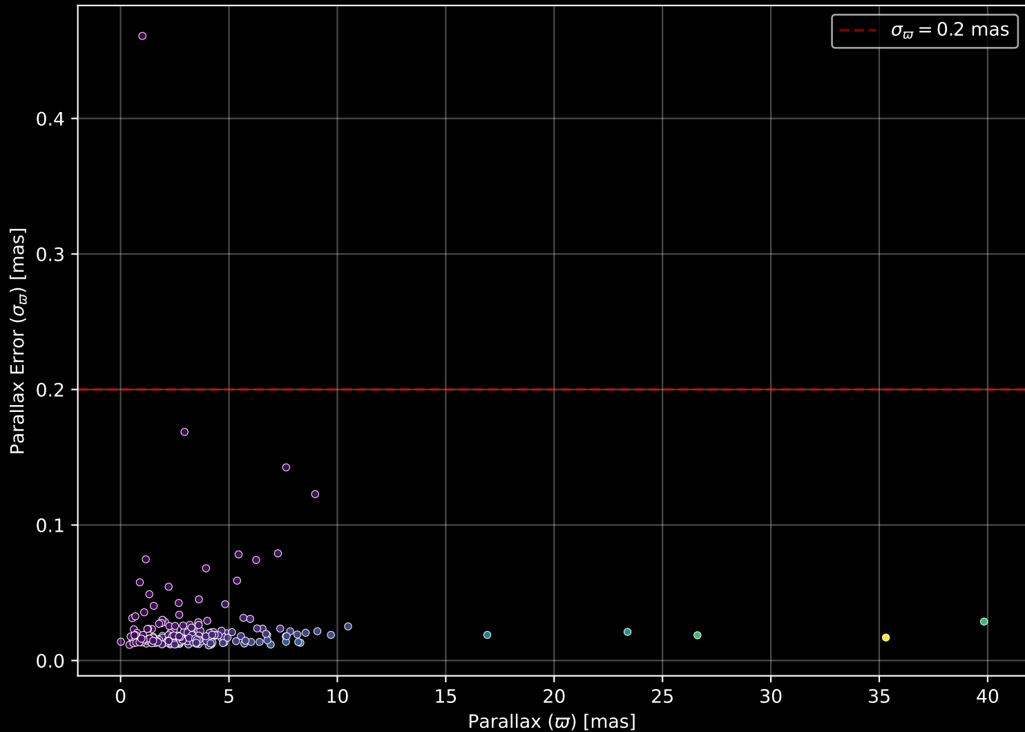
APOGEE DR17 Field: [162+60_MGA] Parallax Quality (n= 205)
