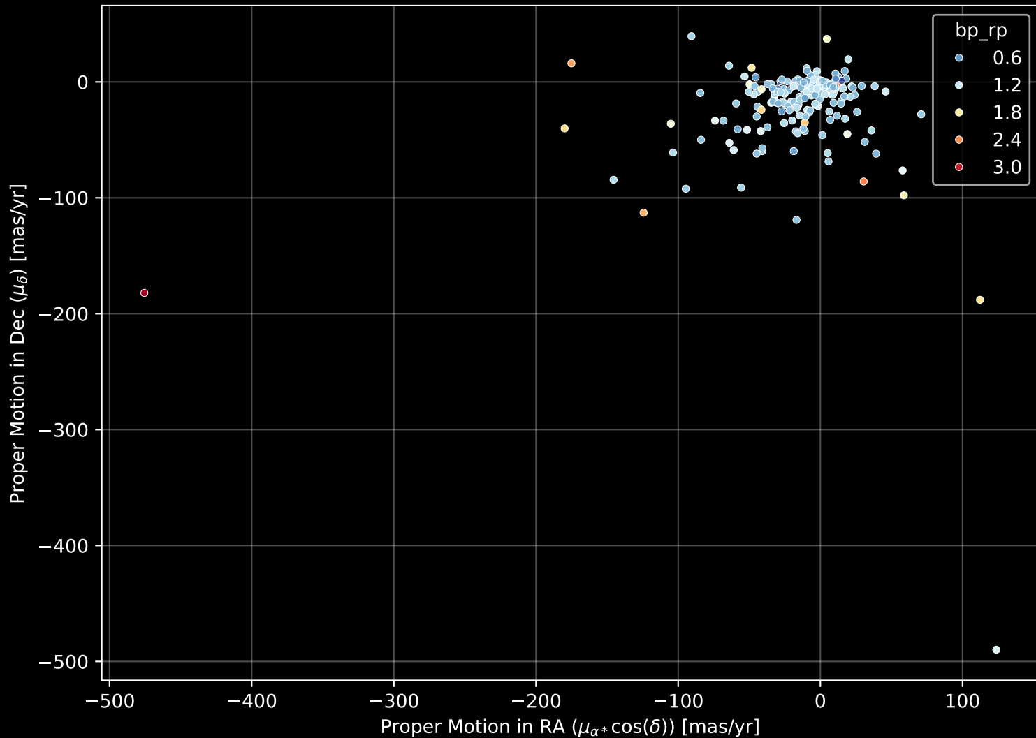
APOGEE DR17 Field: [162+60_MGA] Proper Motion Diagram (n= 205)
