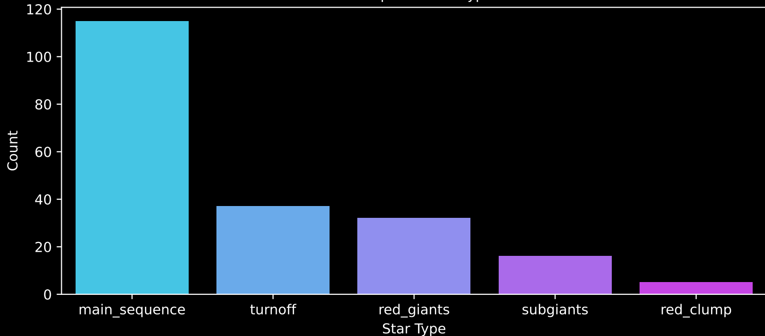
APOGEE DR17 Field: [162+60_MGA] Count plot of Star Type
