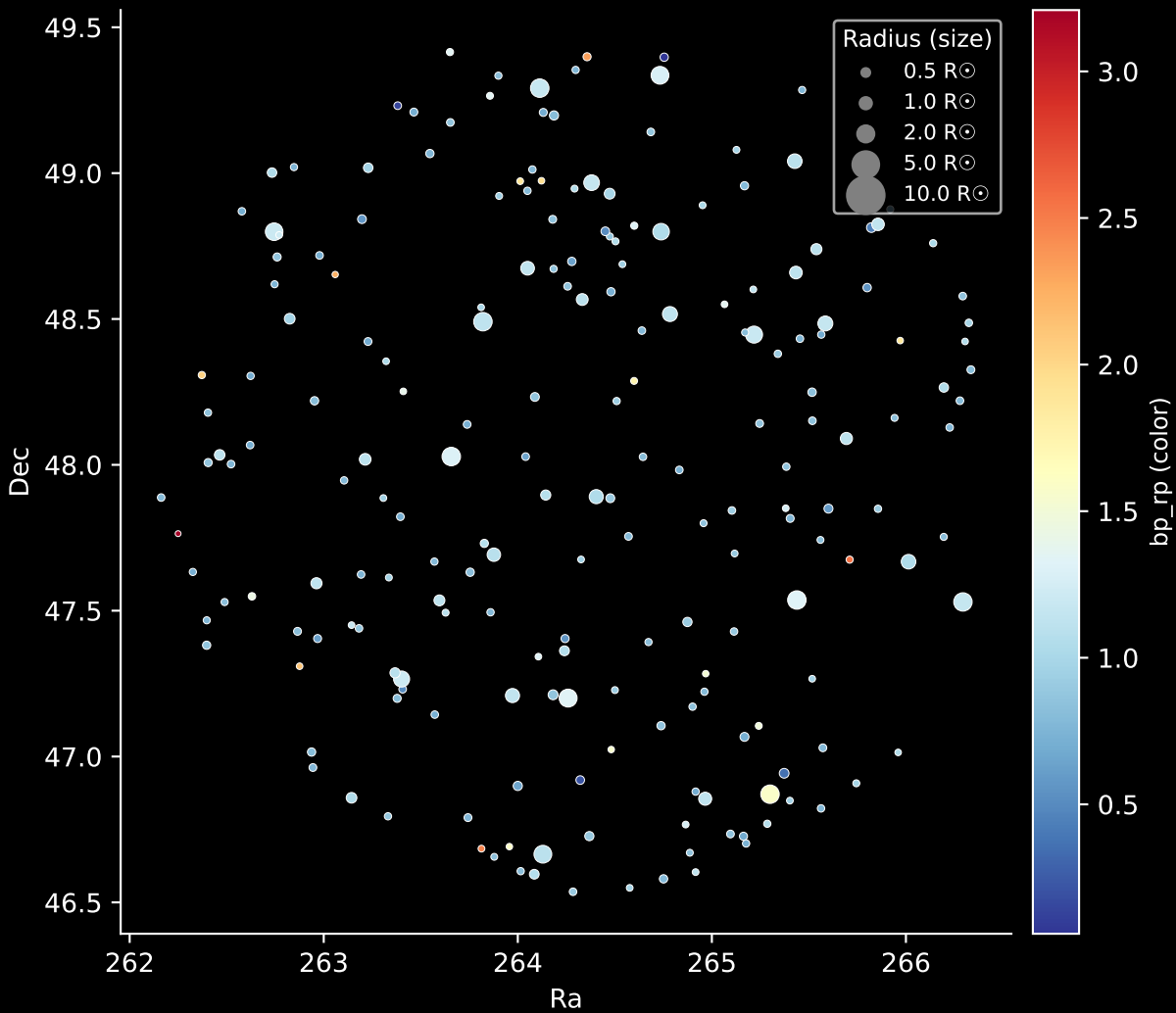
APOGEE DR17 Field: [162+60_MGA] Stars: 205
